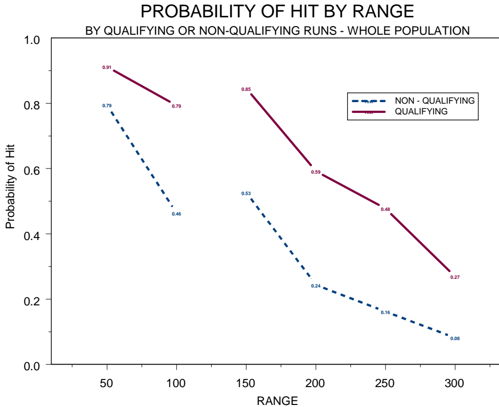
Figure 36. Probability of Hit by Qualifying Iteration
