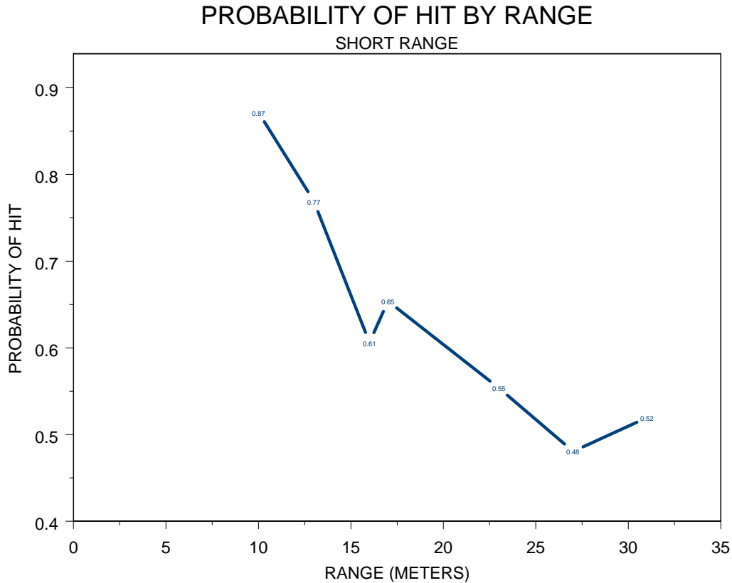
Figure 24. Probability of Hit—Short Range
