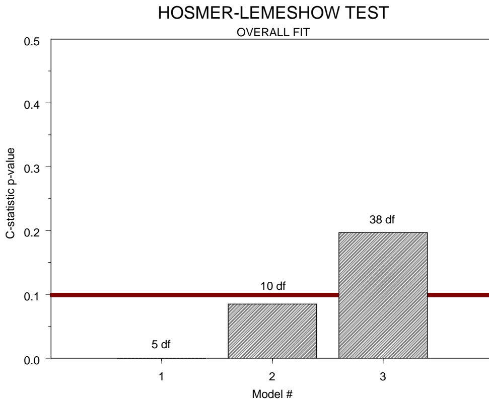
Figure 37. Hosmer-Lemeshow Goodness of Fit Results
