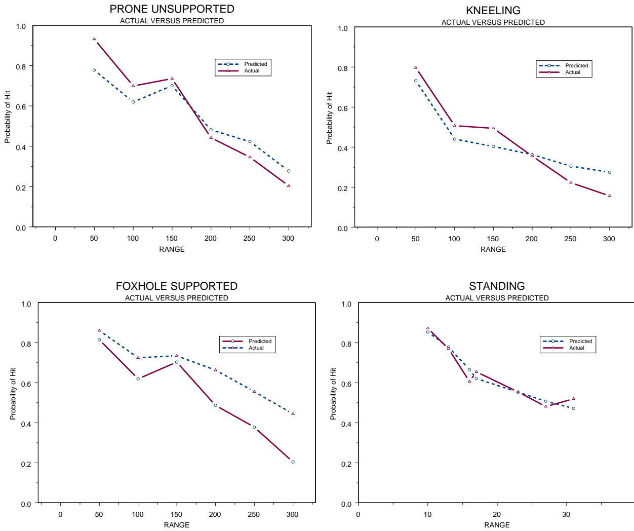
Figure 40. Actual versus Fitted for Posture
