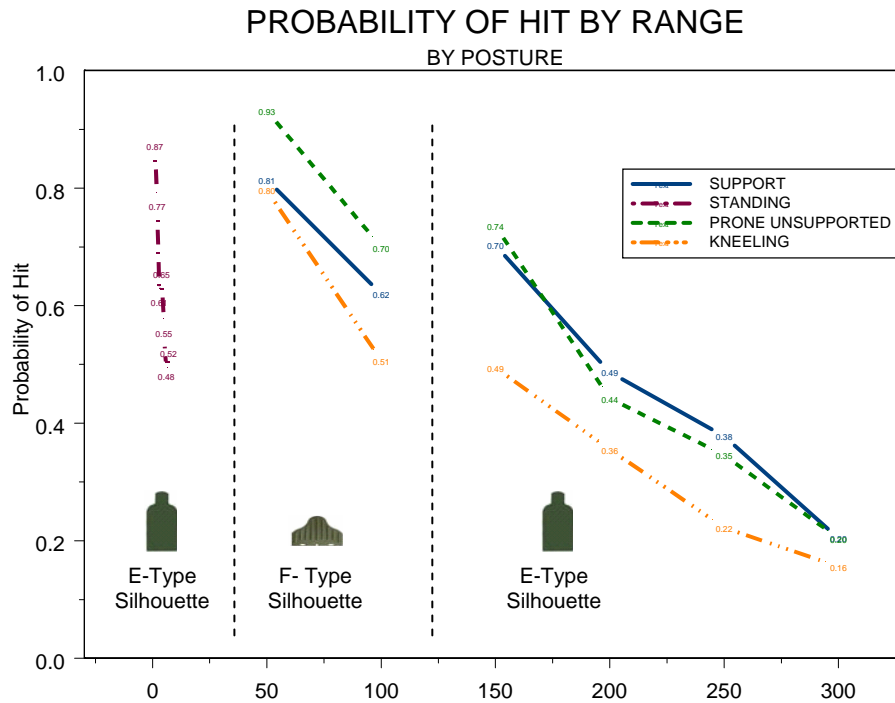
Figure 2. Probability of Hit by Posture
