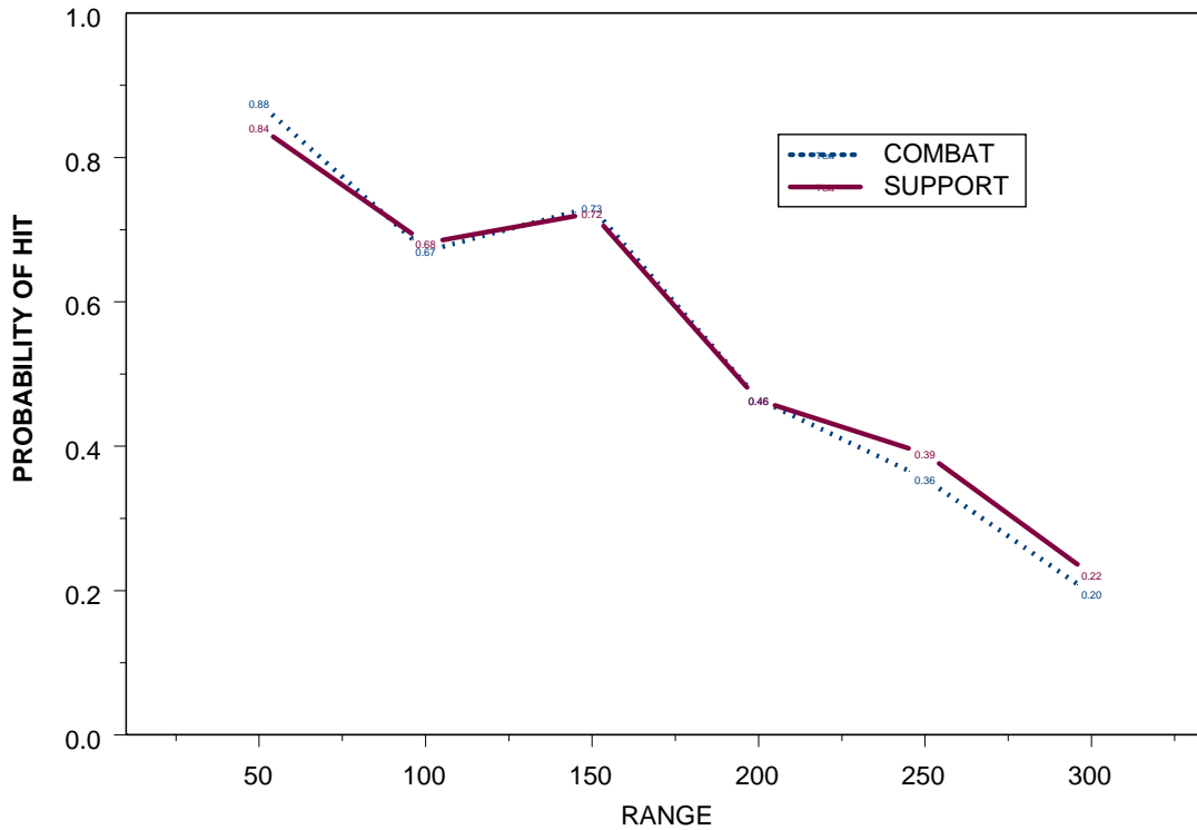
Figure 33. Probability of Hit by MOS Group
