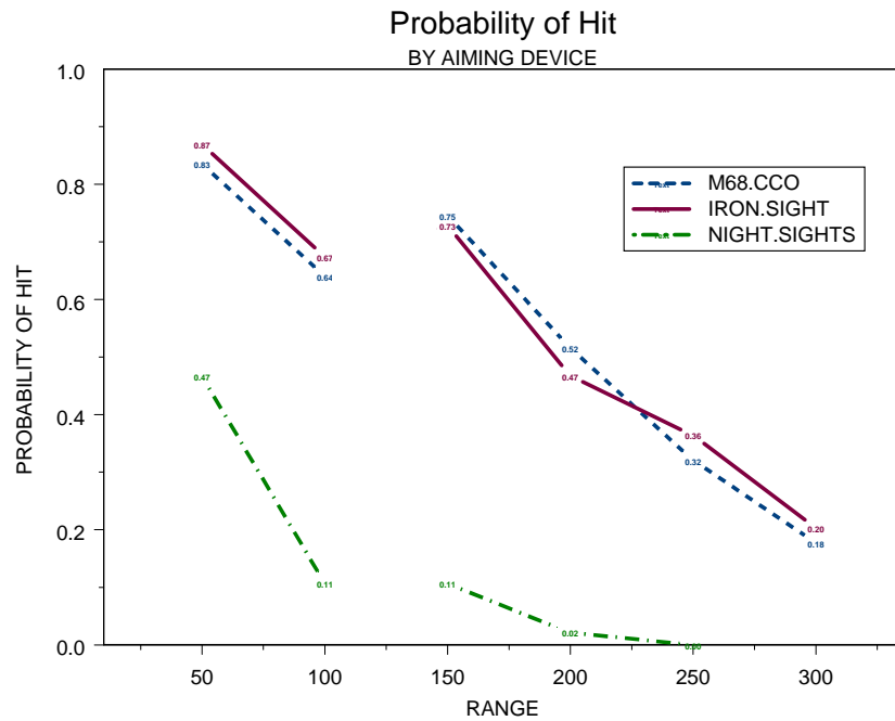
Figure 30. Probability of Hit by Aiming Device—Standard Range
