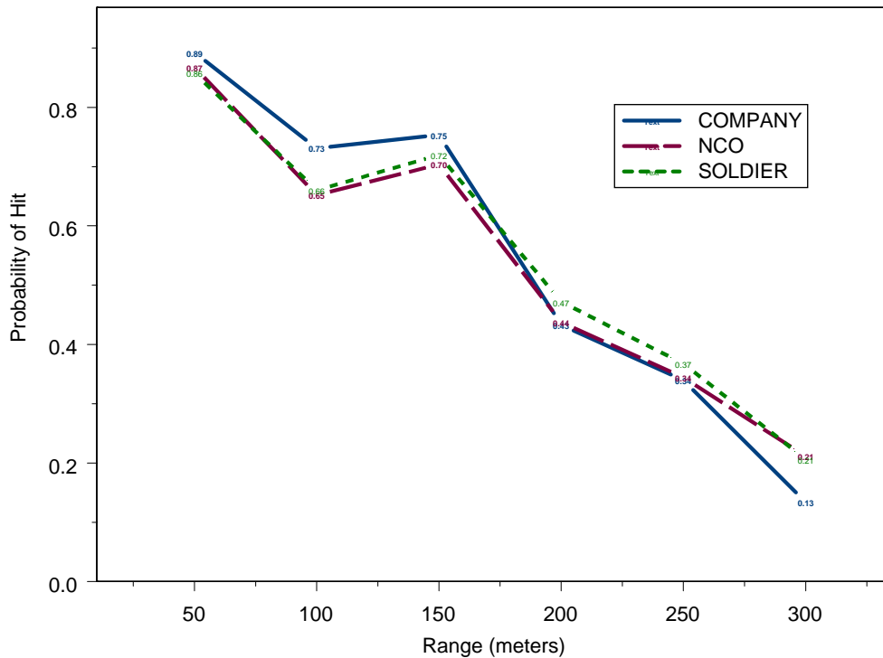
Figure 32. Probability of Hit by Rank Group
