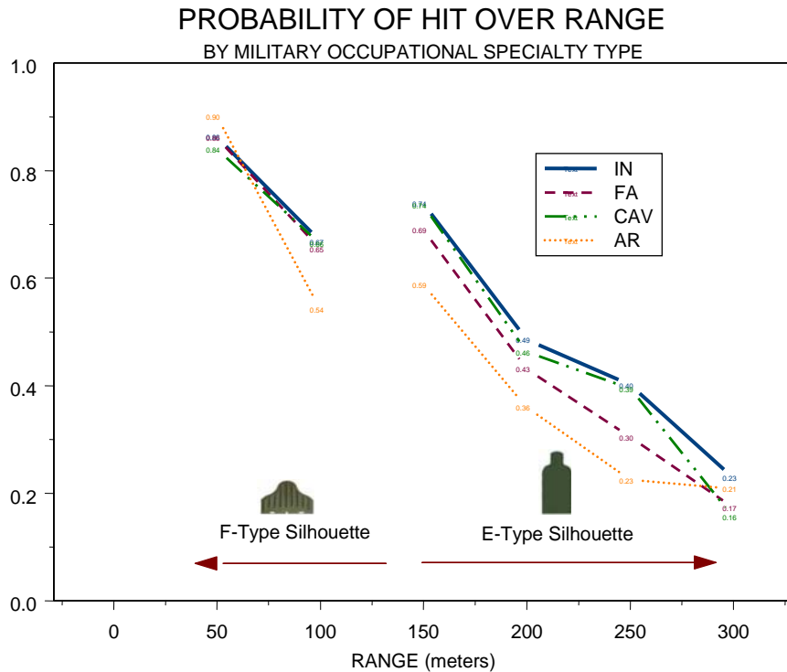
Figure 35. Probability of Hit by Battalion Type
