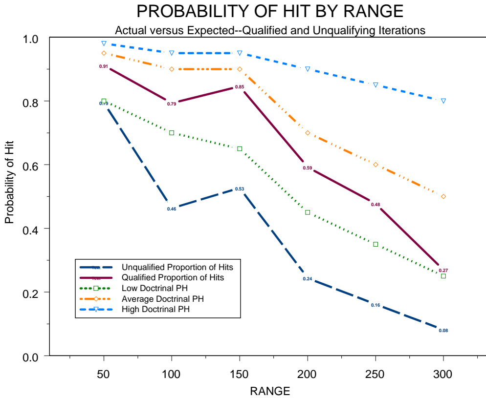
Figure 23. Expected versus Actual Probability of Hit
