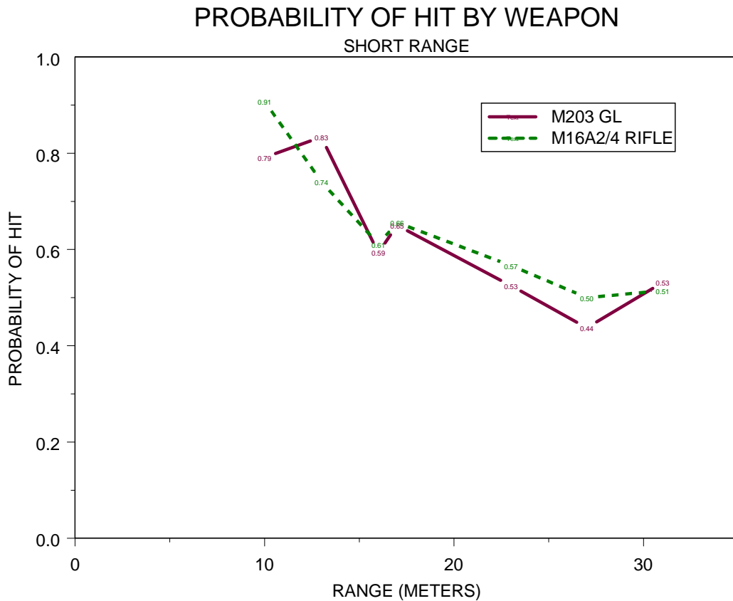
Figure 28. Probability of Hit by Weapon Type—Short Range
