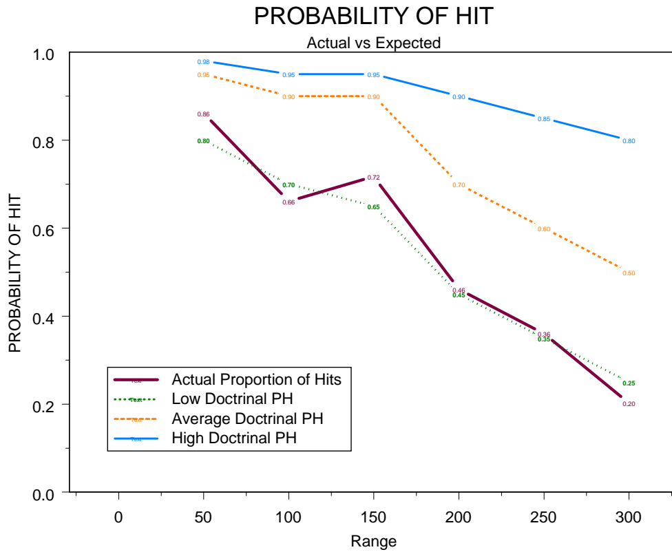
Figure 22. Expected versus Actual Probability of Hit
