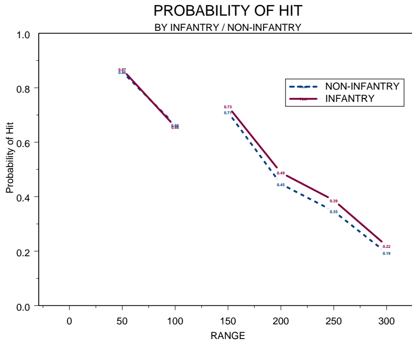
Figure 34. Probability of Hit by Infantry and Non-infantry
