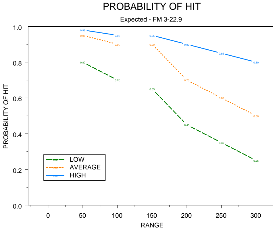
Figure 21. Doctrinal Expected Probability of Hit
