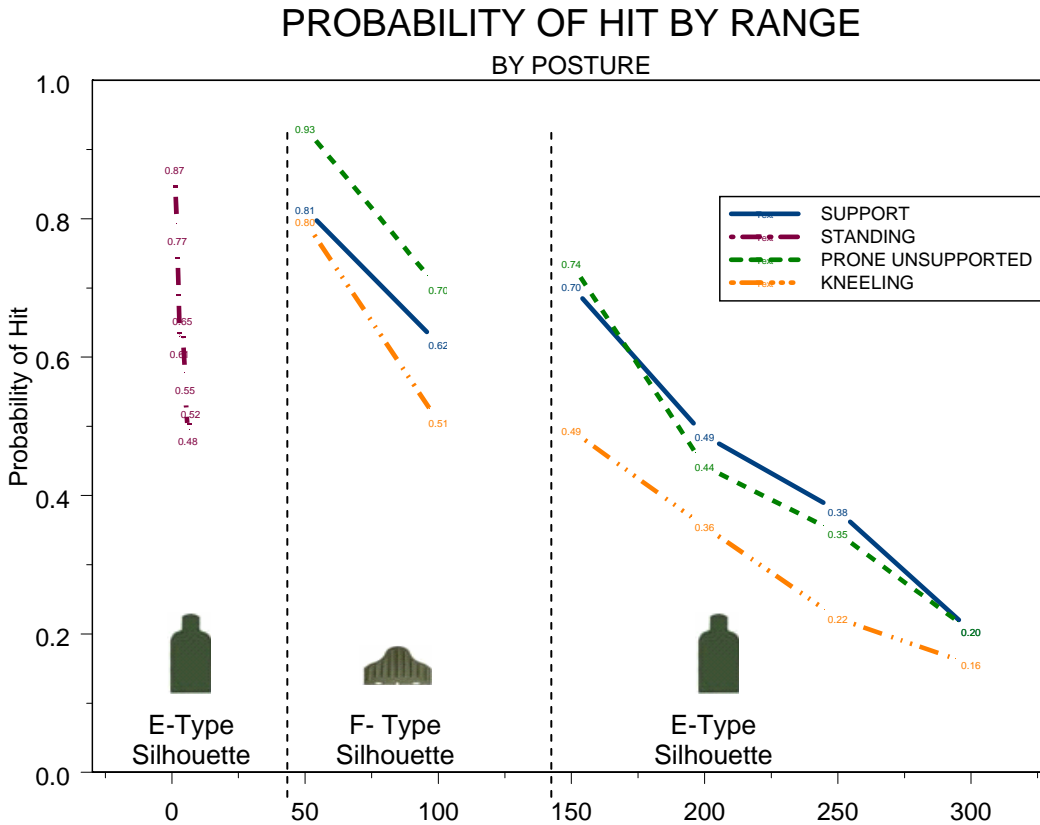
Figure 27. Probability of Hit by Posture
