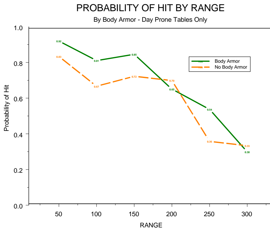
Figure 1. PH by Range and Body Armor Type
