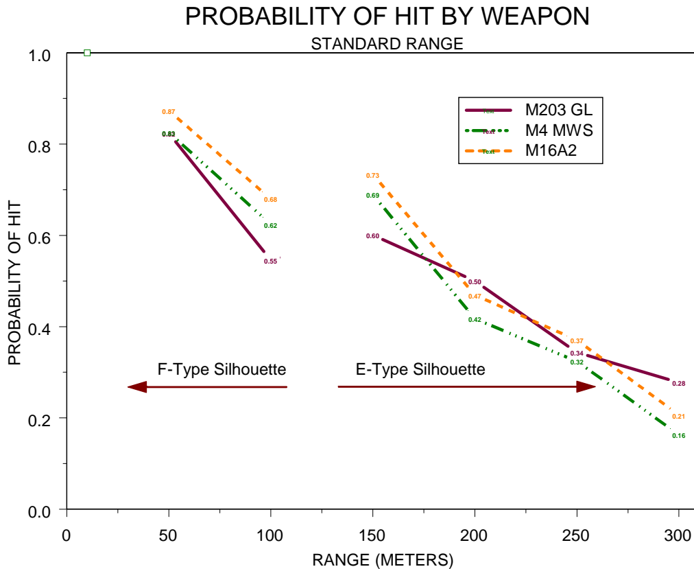
Figure 29. Probability of Hit by Weapon Type—Standard Range
