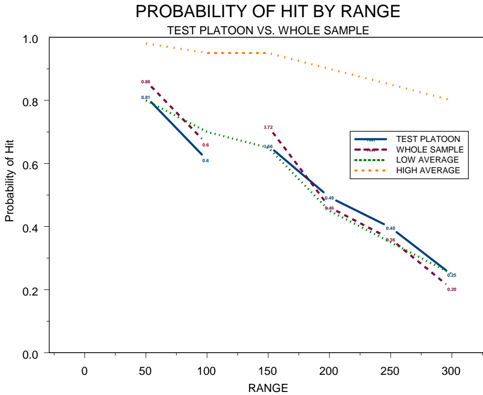
Figure 25. Test Platoon versus Sample Population—Standard Range
