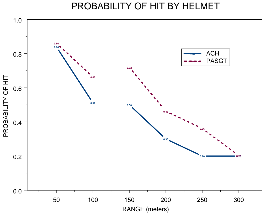
Figure 31. Probability of Hit by Helmet Type
