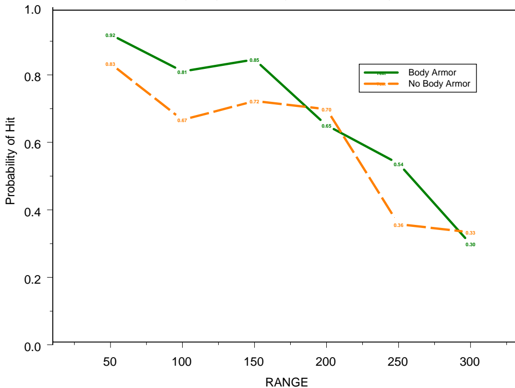
Figure 26. Probability of Hit by Body Armor Type
