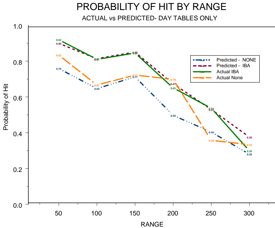
Figure 39. Actual versus Fitted for Body Armor Type—Day Tables Only
