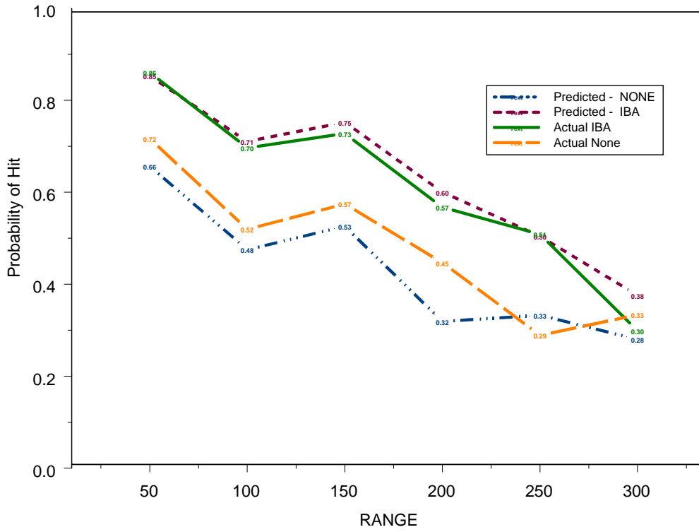
Figure 38. Actual versus Fitted for Body Armor Type
